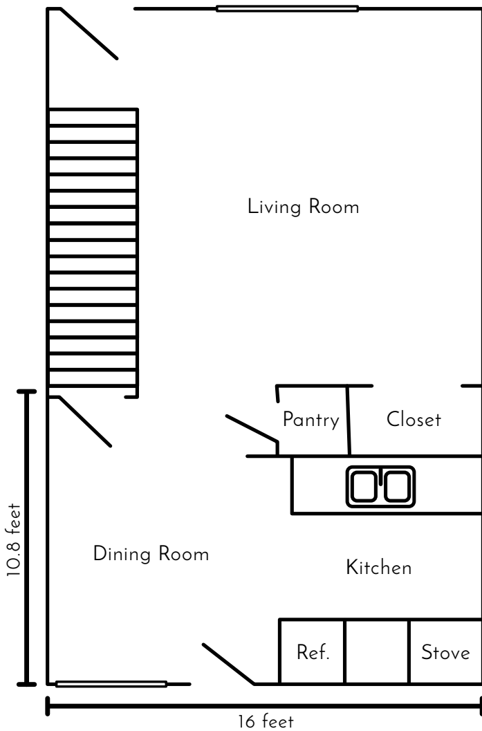
1st Floor
